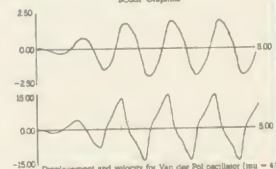
Displacement and velocity for Van der Pol oscillator (mu = 4)
